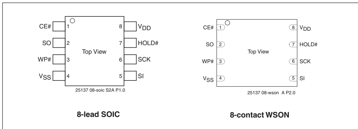
FIGURE 2-1: PIN ASSIGNMENTS
