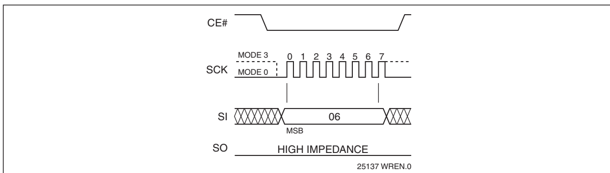
FIGURE 4-15: WRITE ENABLE (WREN) SEQUENCE
